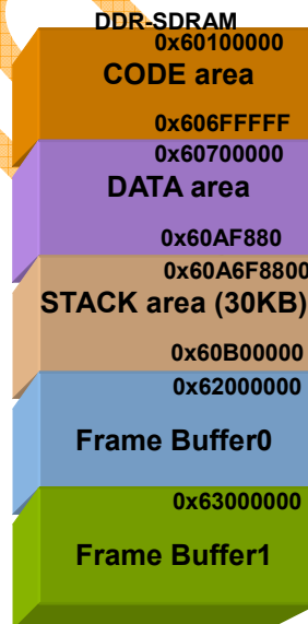
[Fig - 10] DDR-SDRAM base memory map
